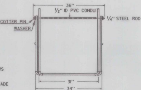
TYPE III (MODIFIED) BARRICADE (STRIPING IS SHOWN WITH TRAFFIC PASSING TO THE RIGHT).
