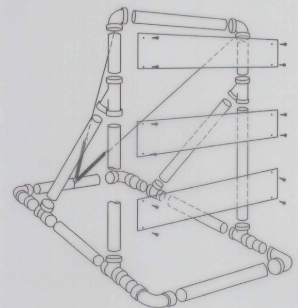
EXPLODED VIEW TYPE III BARRICADE
