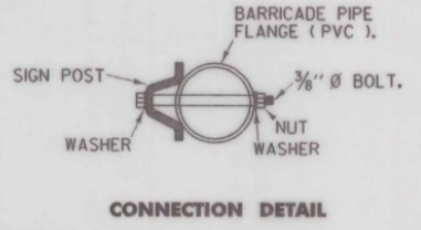
CONNECTION DETAIL
