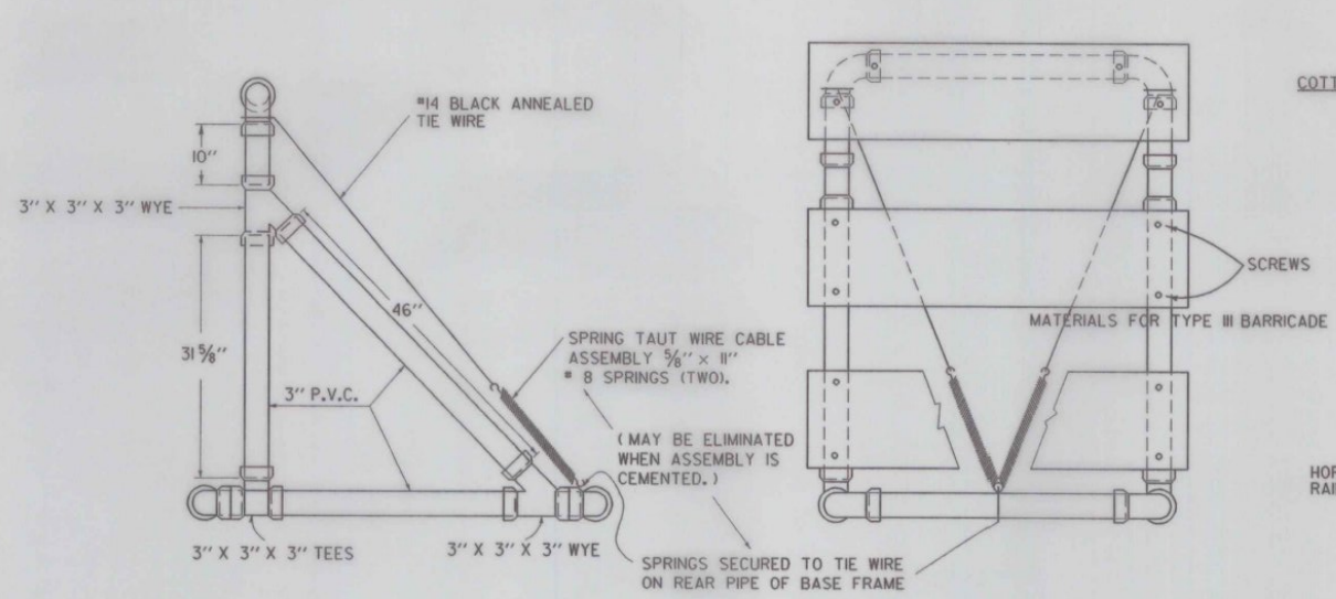
SIDE VIEW TYPE III BARRICADE
