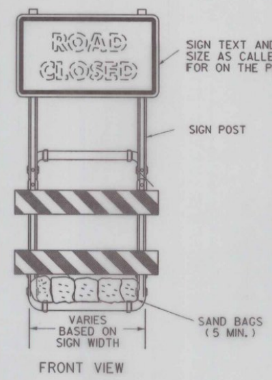
SIGN MOUNTING ON TYPE III BARRICADE (MODIFIED)
