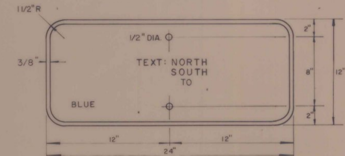
CARDINAL DIRECTION MARKERS FOR USE WITH 24 INCH INTERSTATE ROUTE MARKERS
