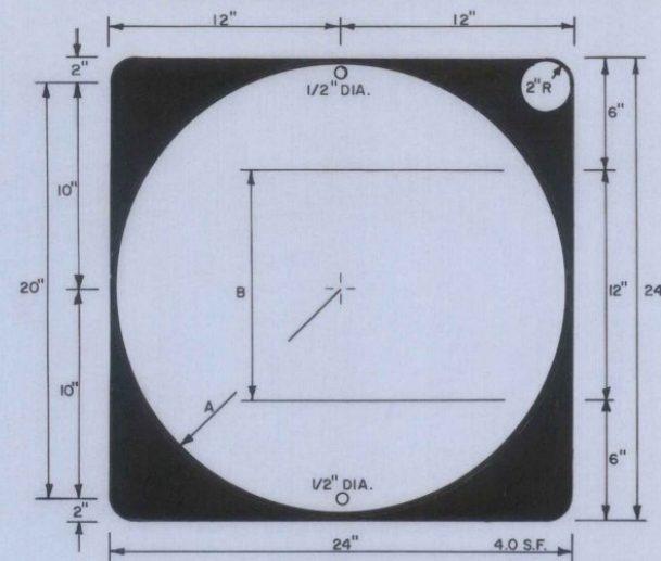
STATE ROUTE MARKER FOR INDEPENDANT USE WITH MARKER ASSEMBLIES
