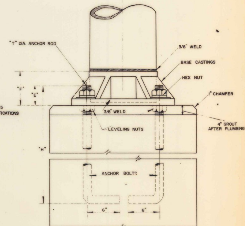
SHOE BASE
