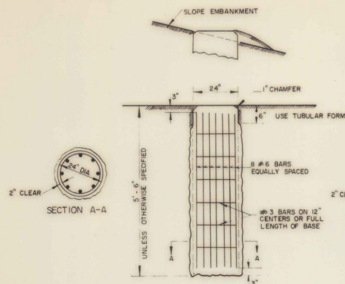
24" DIAMETER "1" FOOTING
