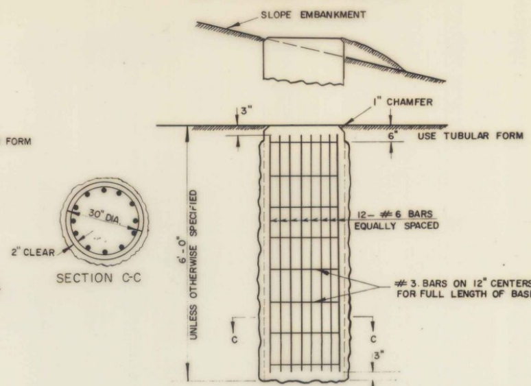
30" DIAMETER "3" FOOTING
