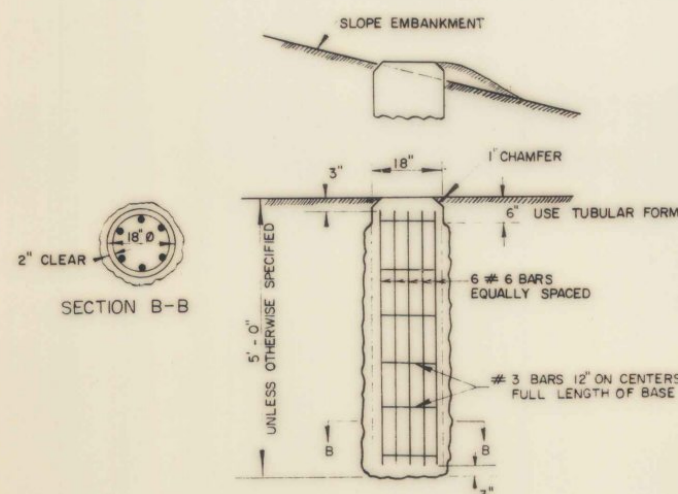
18" DIAMETER "2" FOOTING
