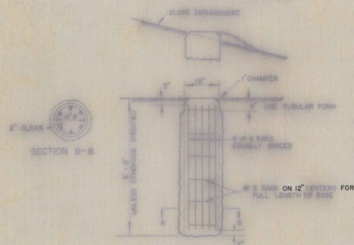
18" DIAMETER #2 FOOTING
