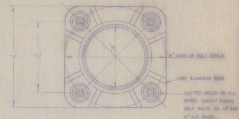
CAST ALUMINUM BASE DETAIL
