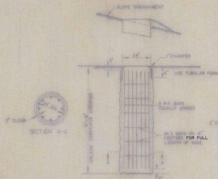
24" DIAMETER #1 FOOTING
