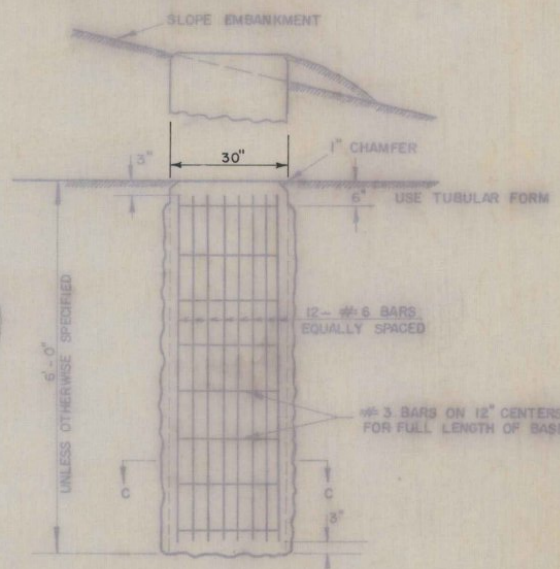
30" DIAMETER #3 FOOTING
