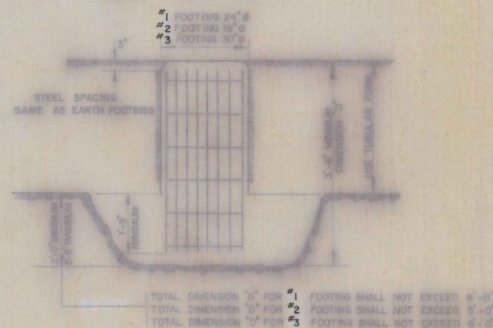
LEDGE FOUNDATION
