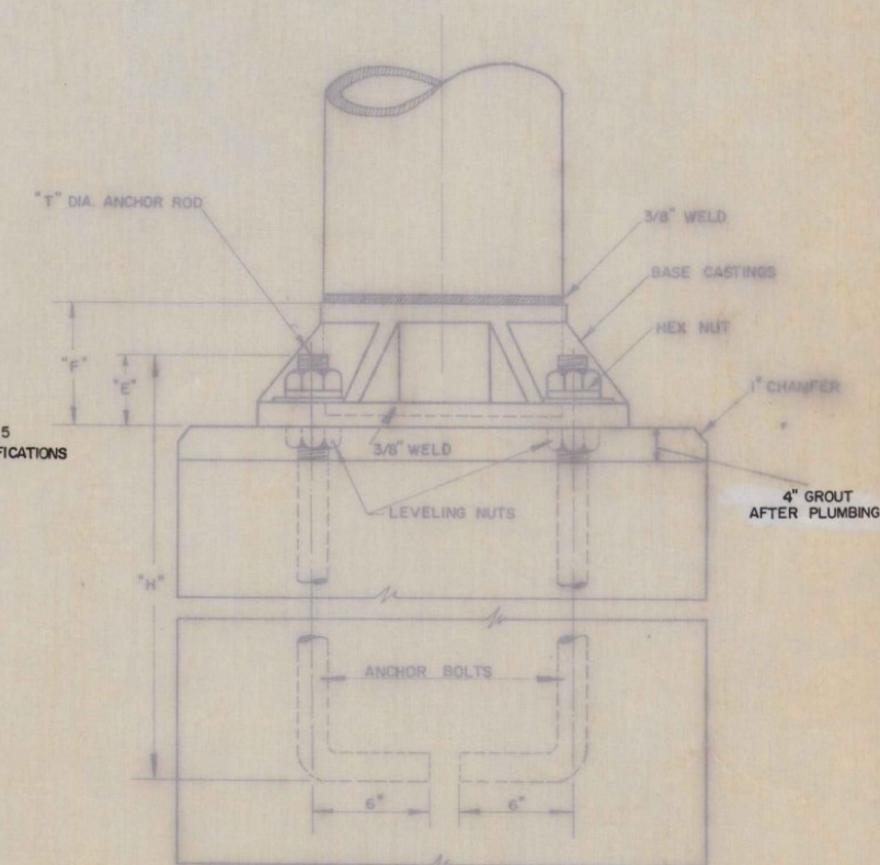
SHOE BASE
