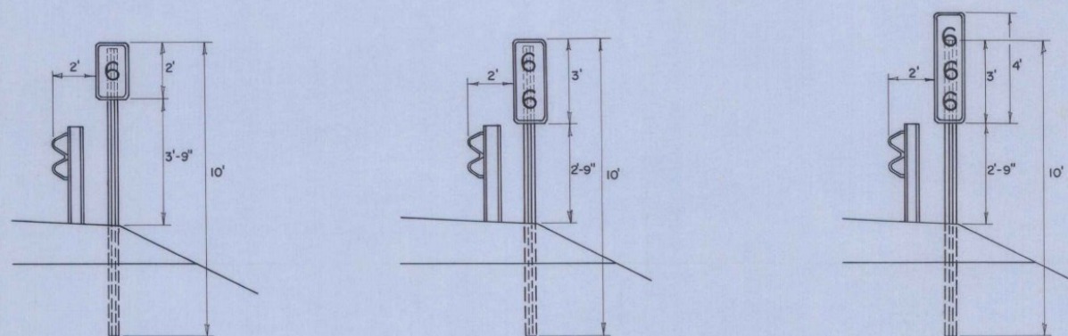
MOUNTING HEIGHTS WITH GUARD RAIL
