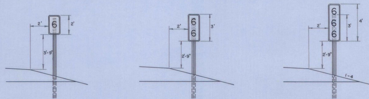
MOUNTING HEIGHTS WITHOUT GUARD RAIL
