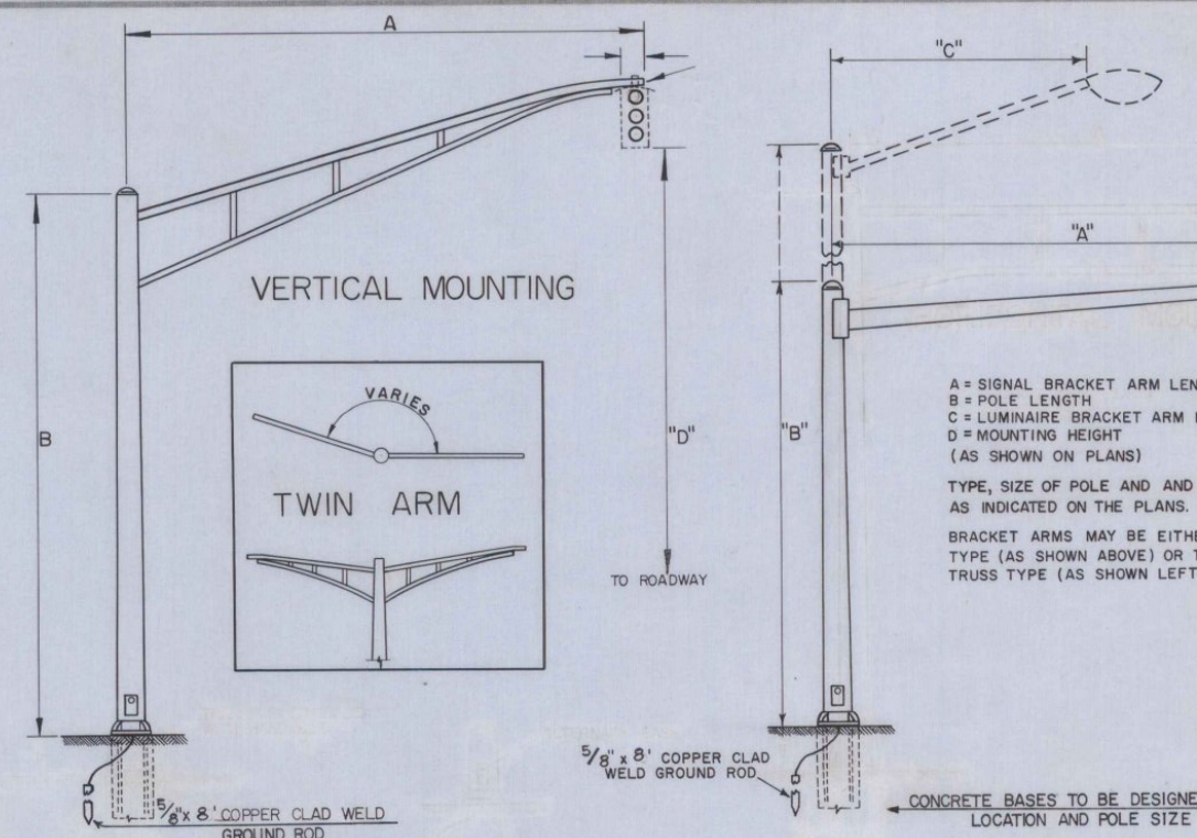
TRAFFIC SIGNAL POLES WITH BRACKET ARMS FOR SIGNALS (AND LUMINAIRES)
