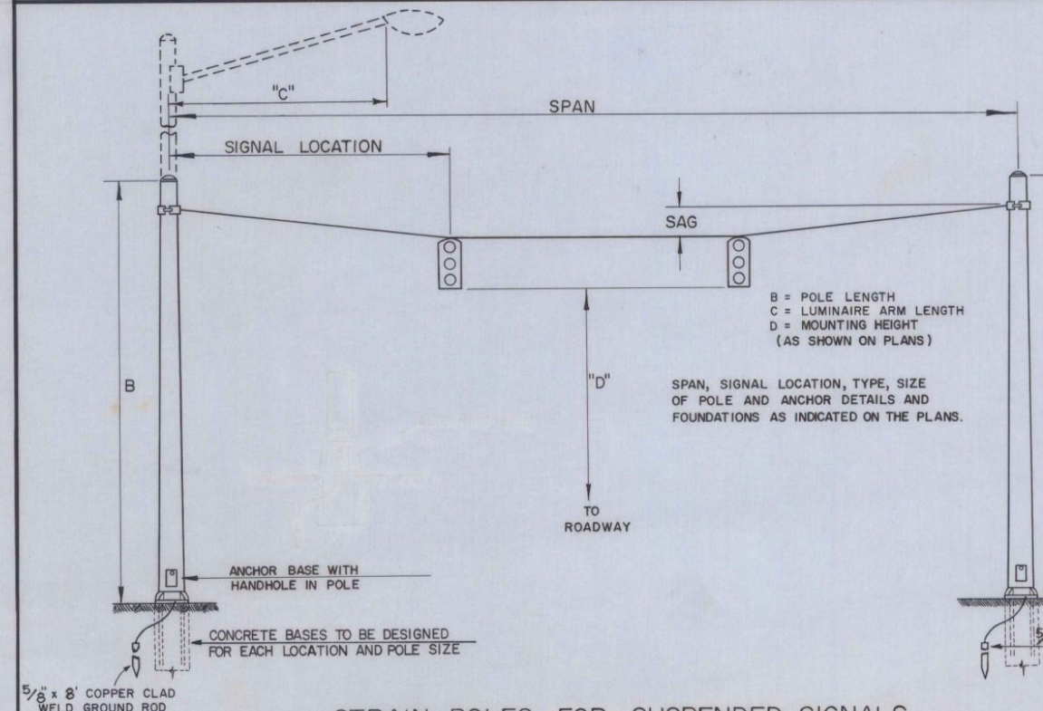
STRAIN POLES FOR SUSPENDED SIGNALS (AND LUMINAIRES)
