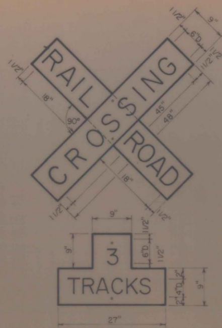
RAILROAD CROSSING SIGN (CROSSBUCK)
