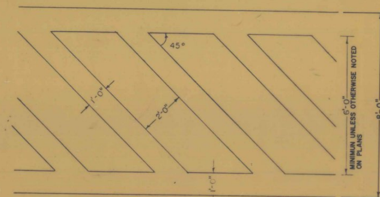
CROSSWALK DETAIL
