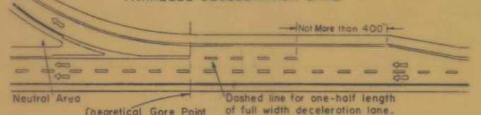
TAPERED DECELERATION LANE
