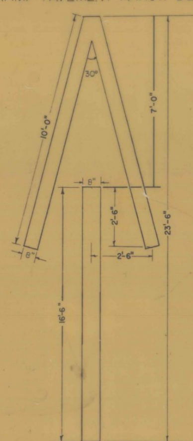
RAMP PAVEMENT ARROW DETAIL
