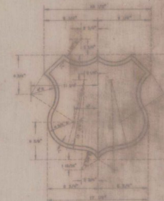
DETAILS OF U.S. SHIELD SYMBOL FOR 24" X 40" ROUTE MARKER.
