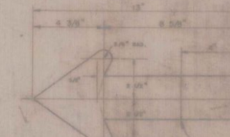
DETAILS OF ARROW FOR USE WITH 24" X 40" ROUTE MARKER.
