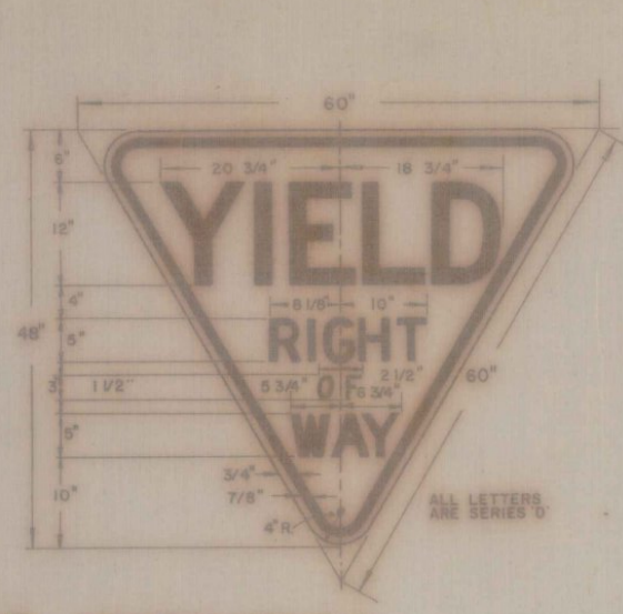
(A) BLACK PAINTED OR SCREENED TEXT ON REFLECTORIZED YELLOW BACKGROUND.
