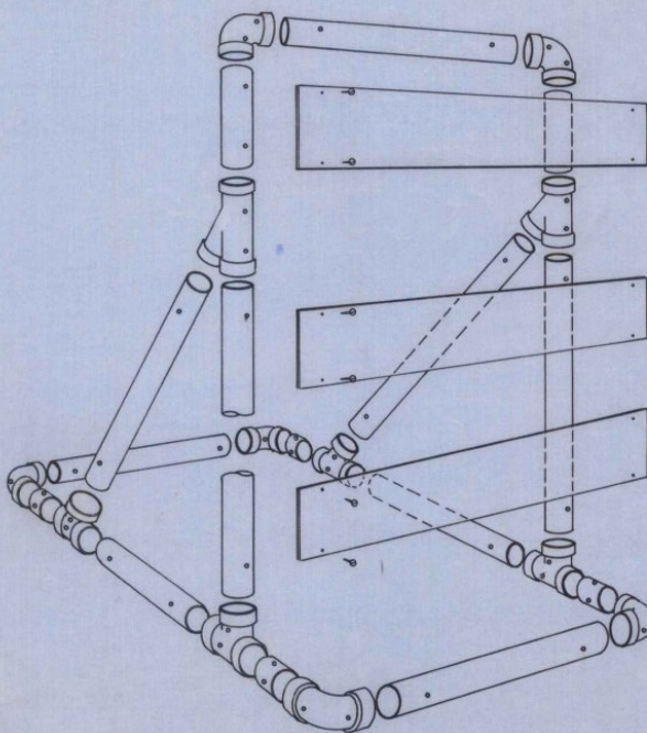
BARRICADE ASSEMBLY
