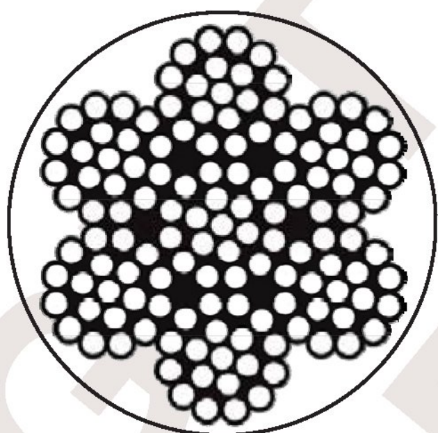
7 x 19 Steel Core
