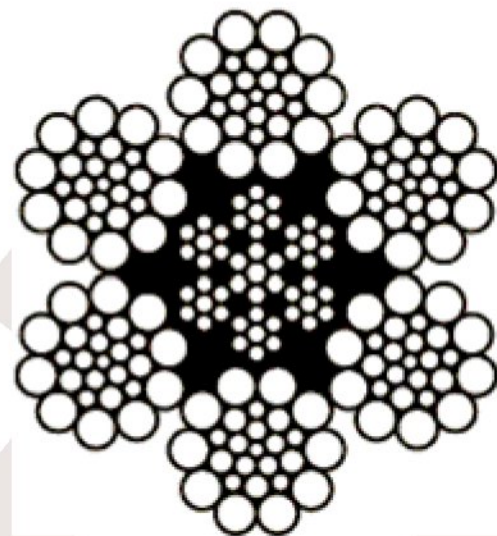
6 x 26 Warrington-Seale IWRC
