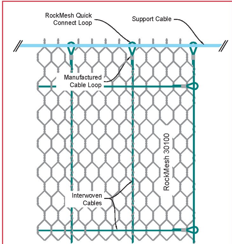
Detail C.2.A - Panel to Support Cable Connection - With RockMesh Quick Connect Cable Loop Option -
