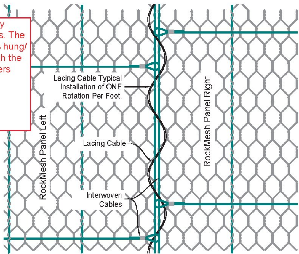
Detail C.1.A - Panel to Panel Connection - With Wire Rope Lacing Option -
