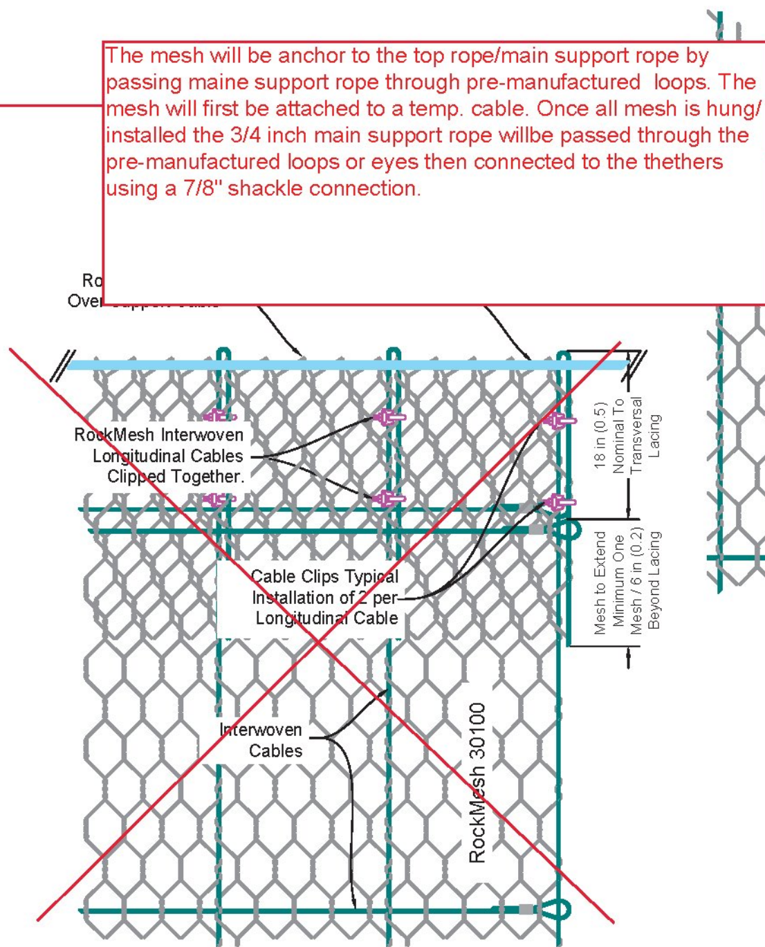
Detail C.2.B - Panel to Support Cable Connection - With Wire Rope Clip Option -
