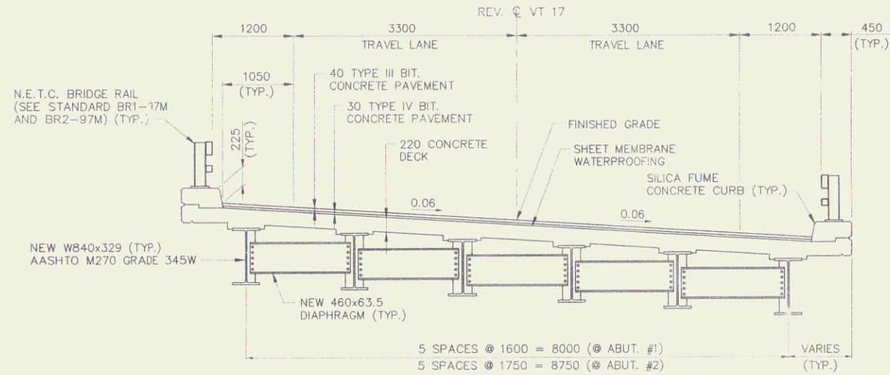
BRIDGE TYPICAL SECTION
