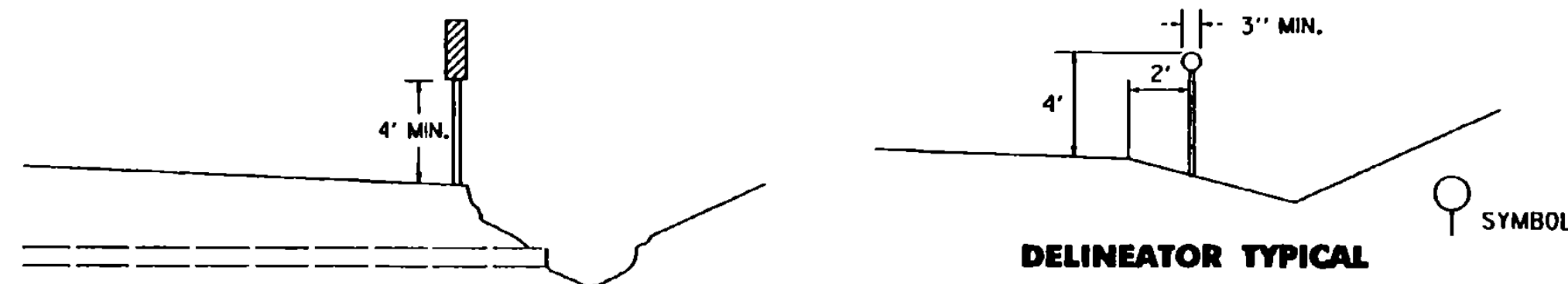
DELINEATOR TYPICAL
