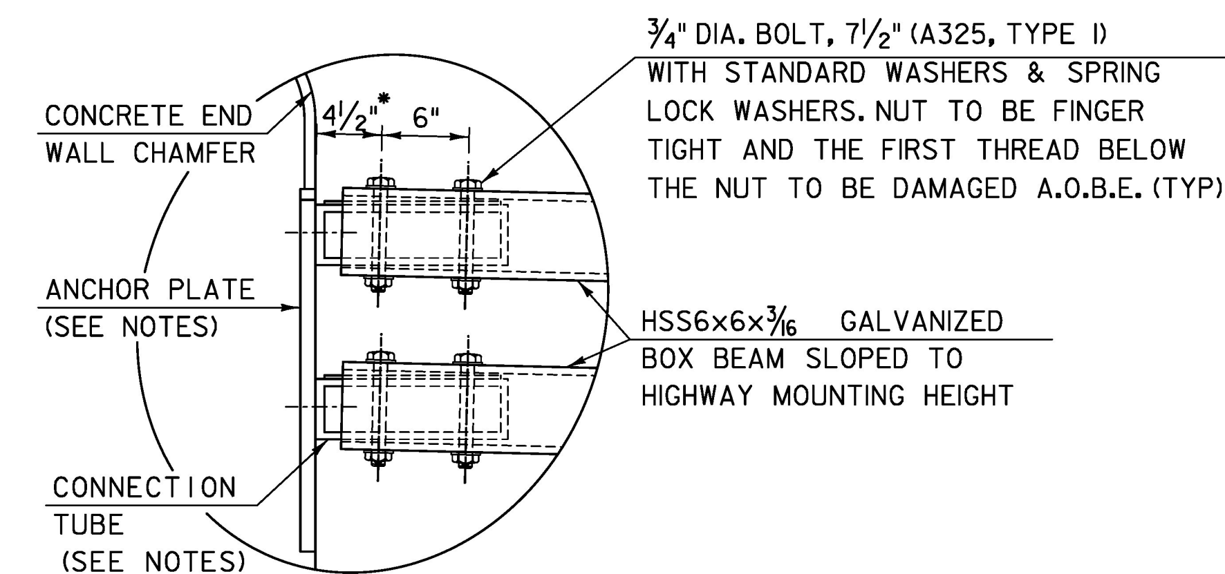
DETAIL "A" NOT TO SCALE * AT 68°F
