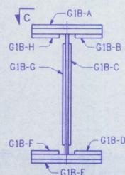
SECT. A-A FOR G1B (G2B-G6B SIMILAR)
