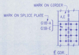
VIEW C
