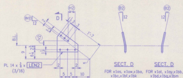
LATERAL GUSSET PLATES
