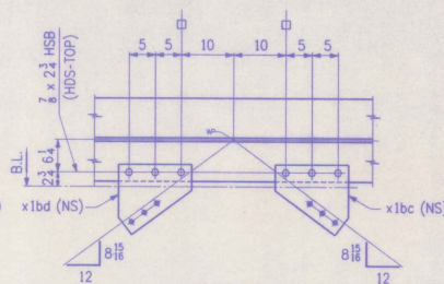
SECT. B2 (DEVELOPED)
