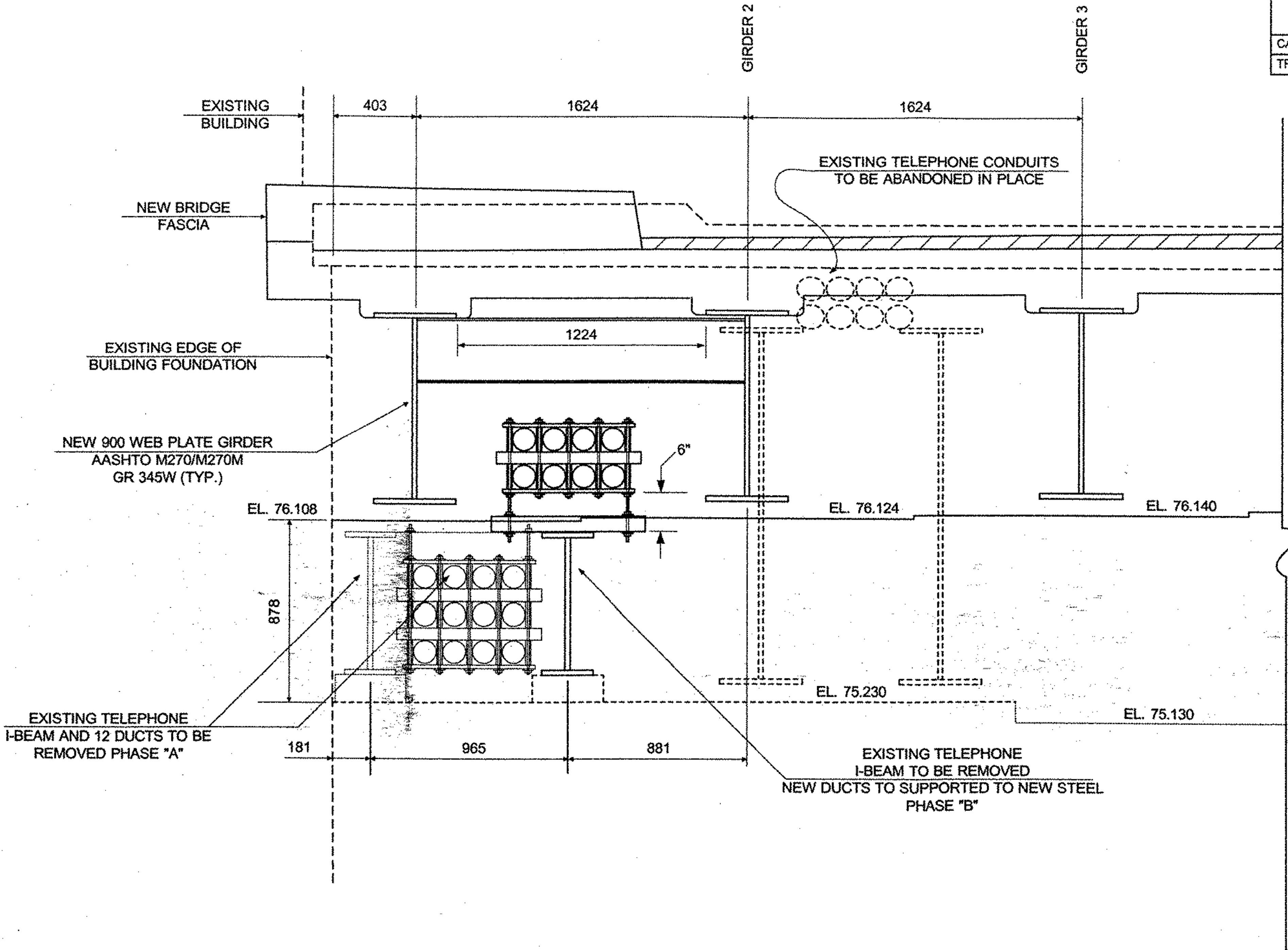
EXISTING AND PROPOSED TELEPHONE FACILITIES @ ABUTMENT NO. 2, LEFT SIDE PHASE "A"
