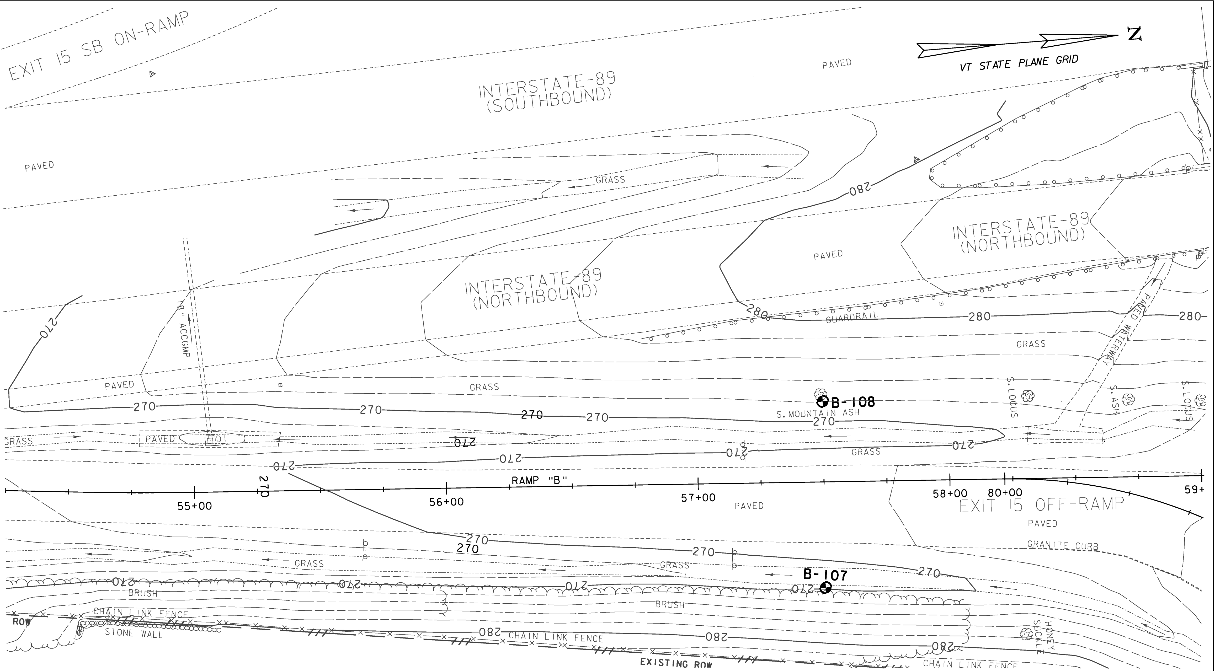
BORING LAYOUT
