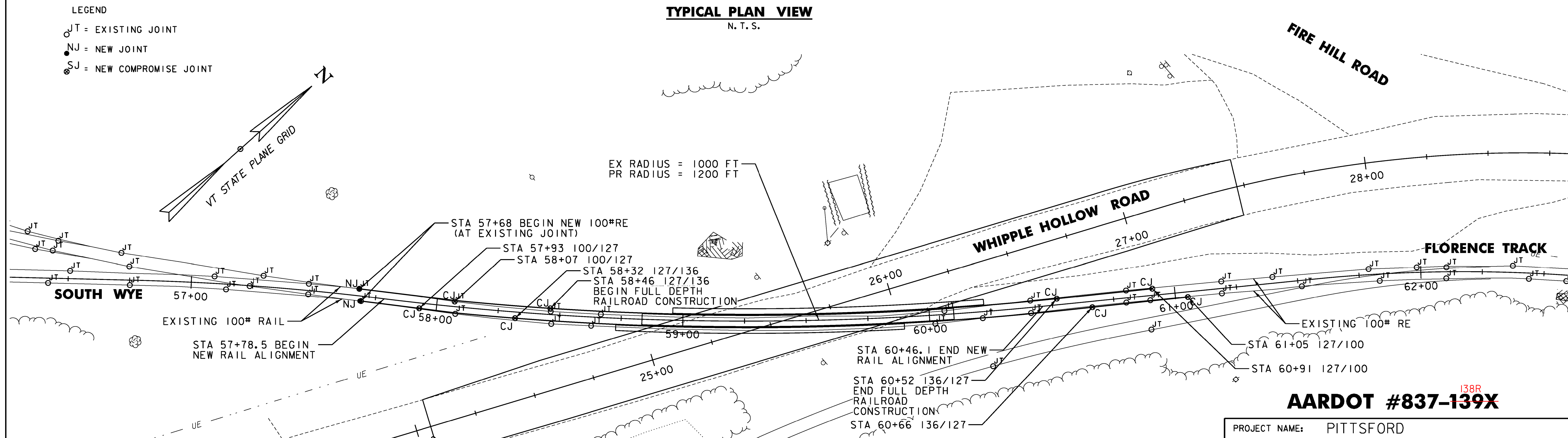
EXISTING AND PROPOSED RAIL JOINT LAYOUT
