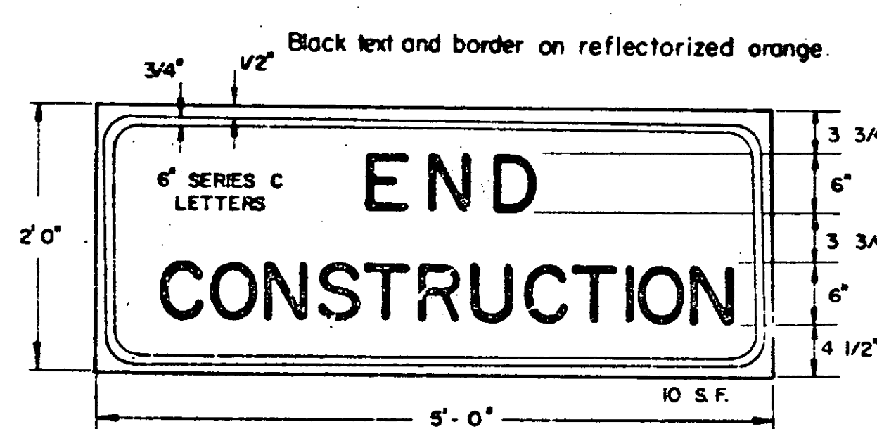
SIGN B-7 (STD. G 20-2)
