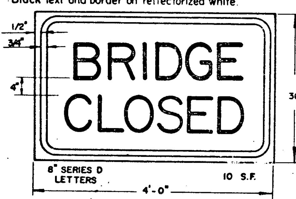
SIGN B-5 (STD. R 11-2 MODIFIED)
