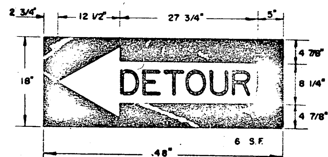
SIGN No. B-6 (STD. W 4-10)
