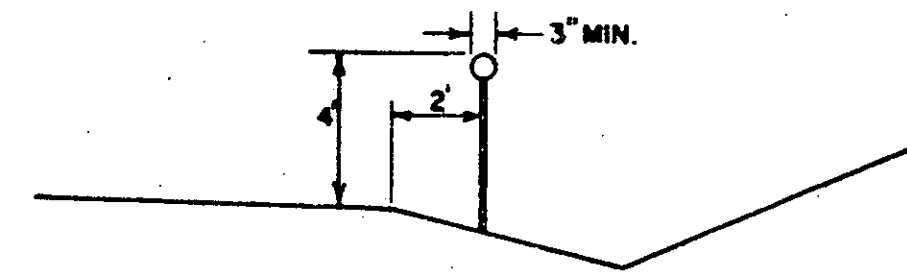
DELINEATOR TYPICAL
