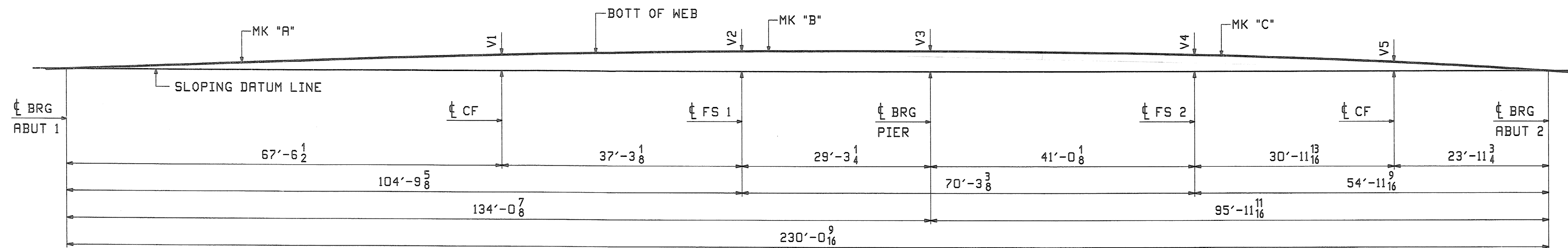
SHOP REAMING DIAGRAM
