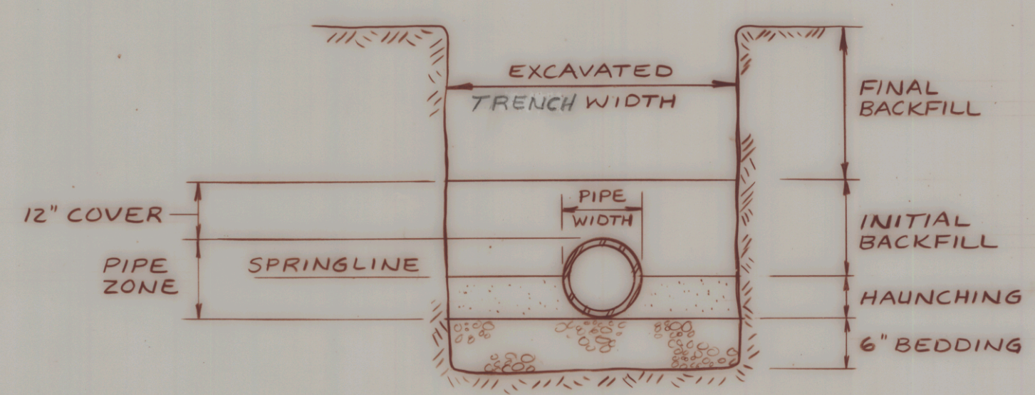
△ TYPICAL TRENCH DETAIL FOR PVC PIPE NO SCALE
