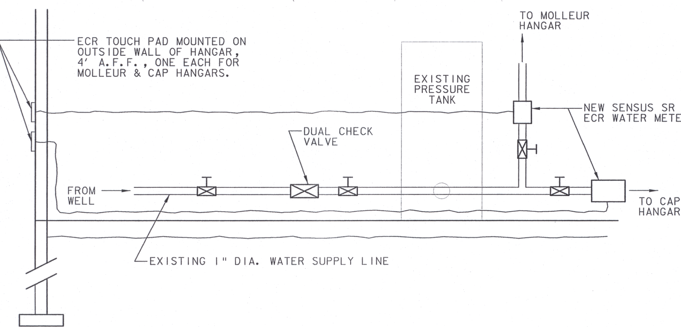
(C) 2 WATER METER IN UTILITY ROOM SCALE: NONE
