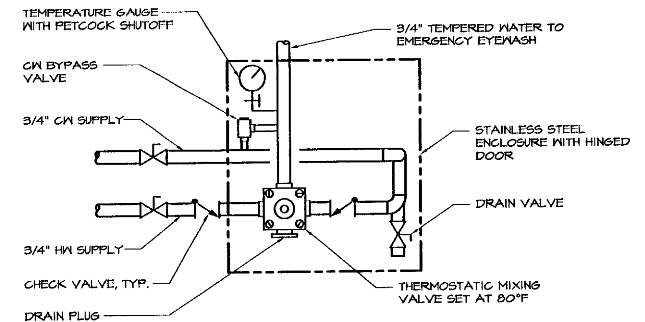
EYEWASH MIXING VALVE DETAIL NOT TO SCALE
