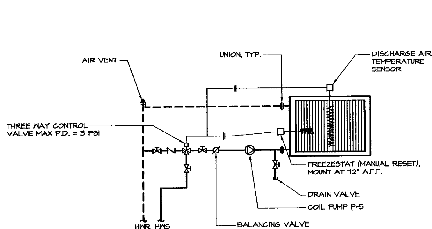
HOT WATER COIL HC-1 PIPING DETAIL NOT TO SCALE
