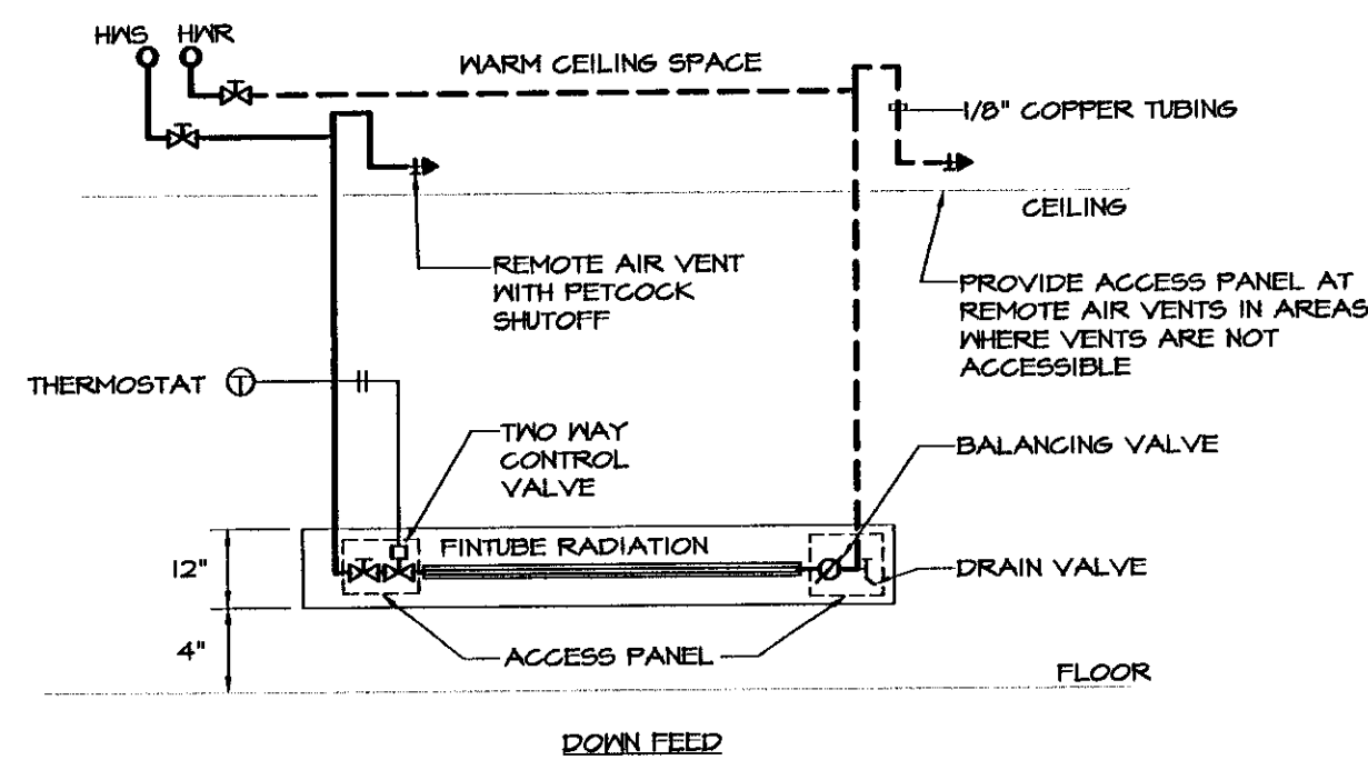
RADIATION PIPING DETAILS NOT TO SCALE
