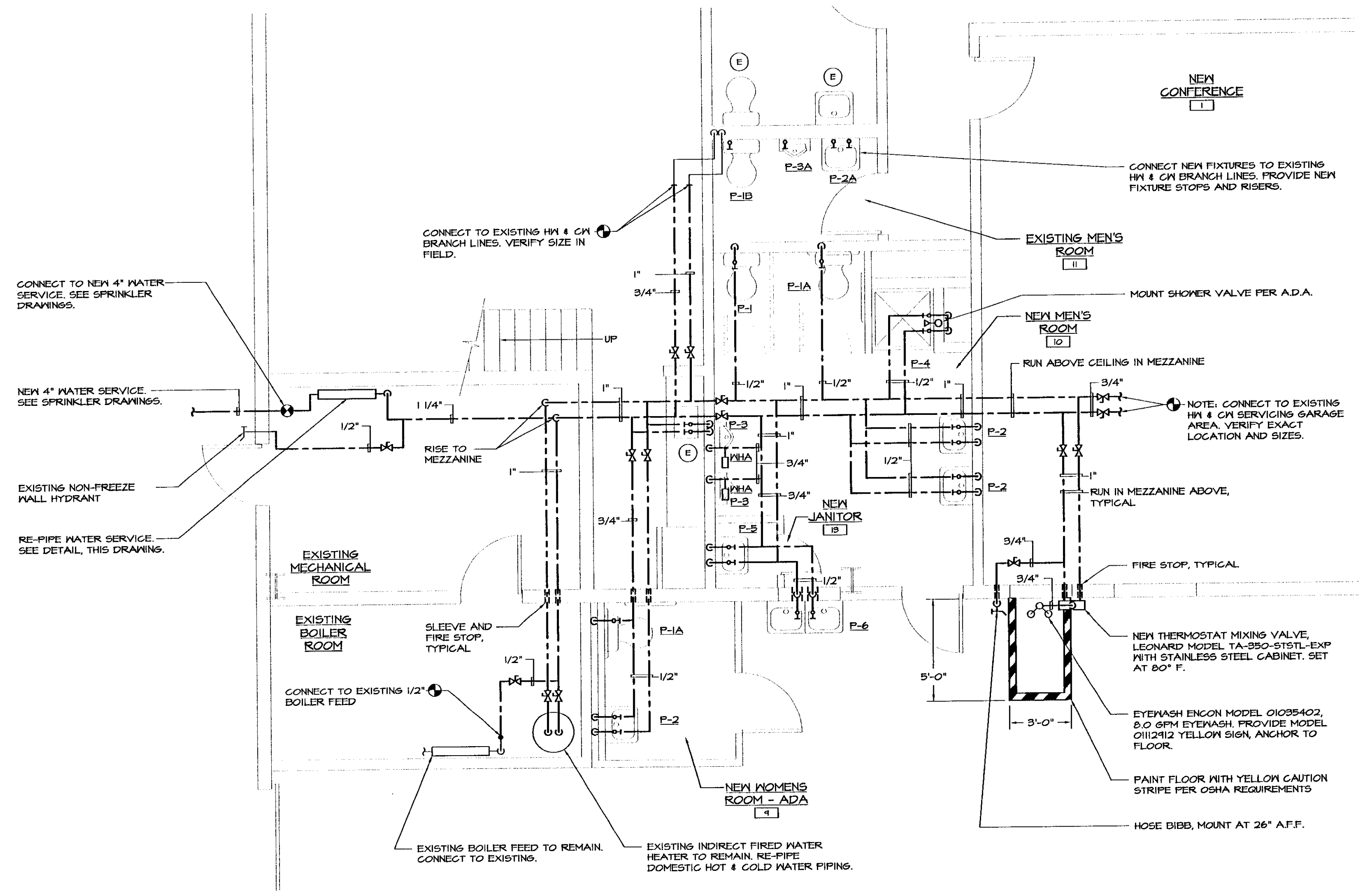
PARTIAL MAIN FLOOR PLAN - DOMESTIC WATER SCALE: 1/4"=1'-0"
