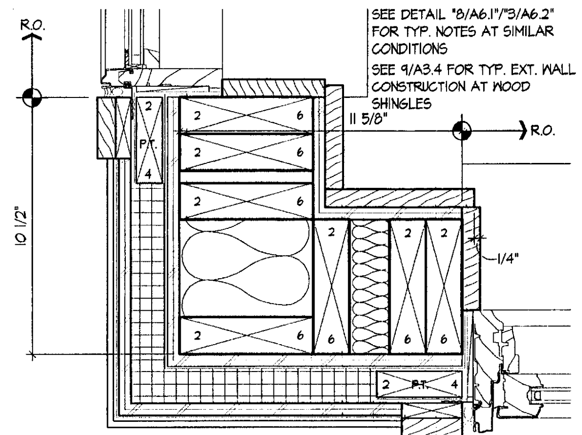
6 FIXED WINDOW JAMB/DORMER #2 SCALE: 3" = 1'-0"
