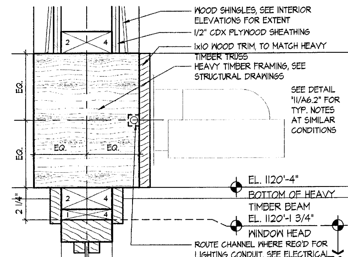
12 INTERIOR WINDOW HEAD SCALE: 3" = 1'-0"
