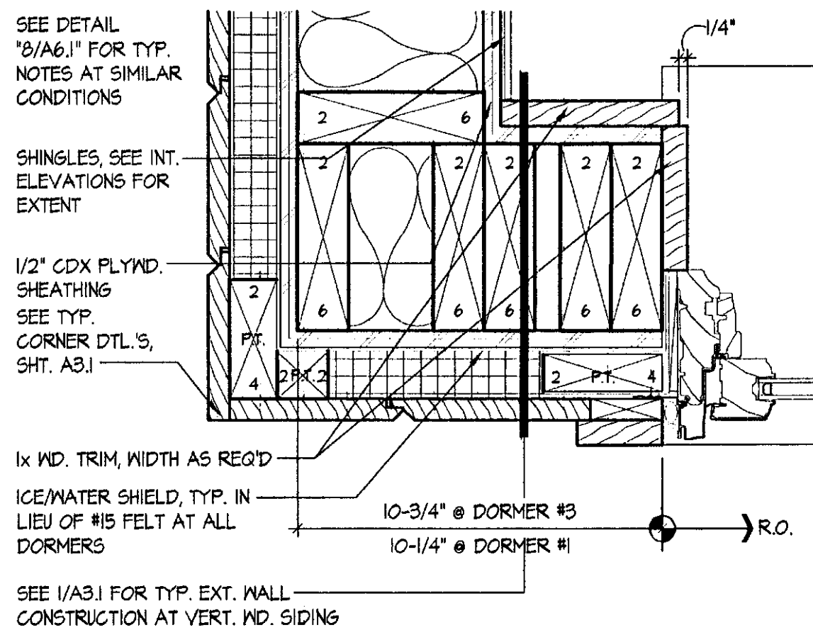
3 FIXED WINDOW JAMB/DORMER #1, #3 SCALE: 3" = 1'-0"
