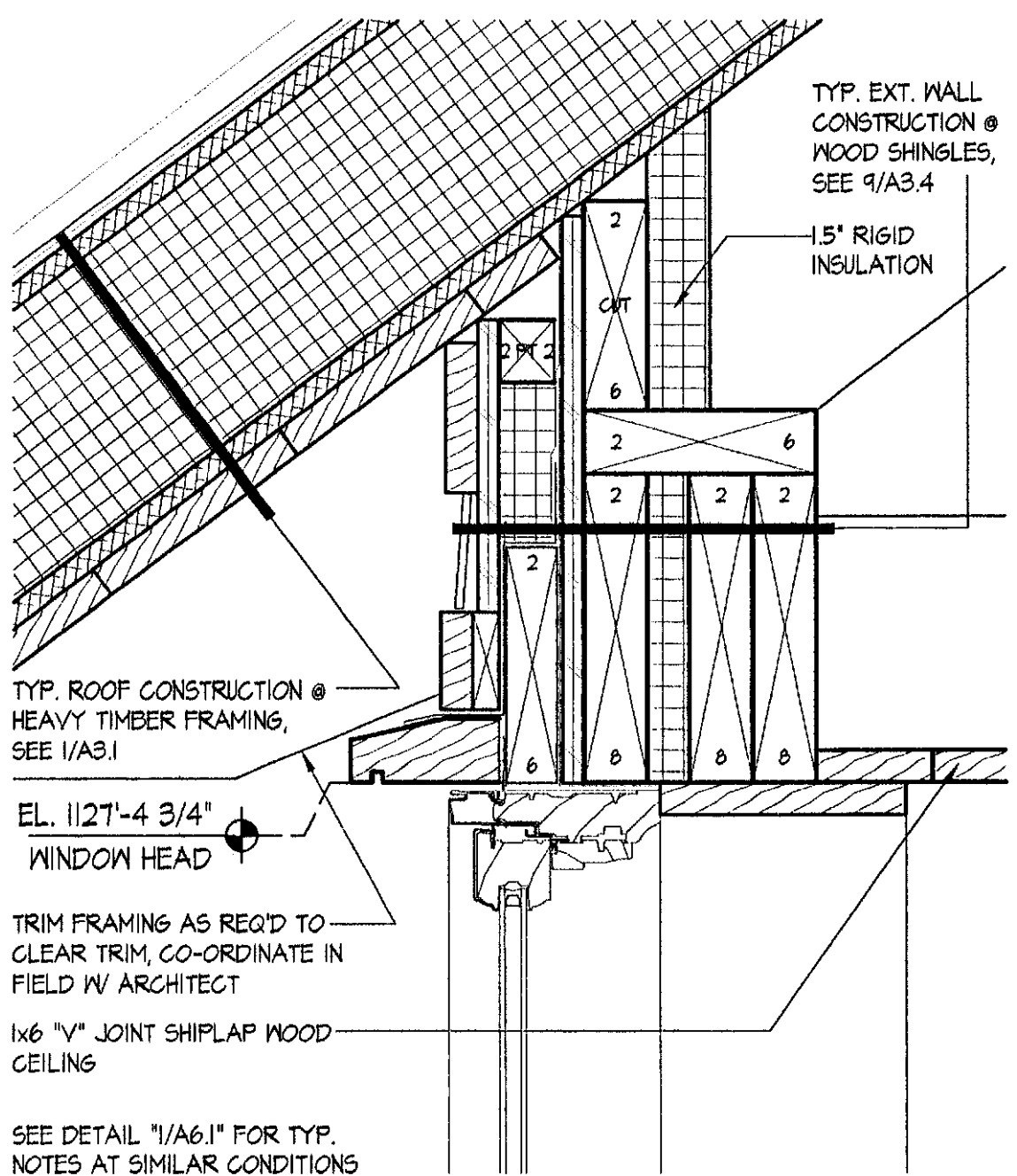
2 FIXED WINDOW HEAD @ DORMER SCALE: 3" = 1'-0"
