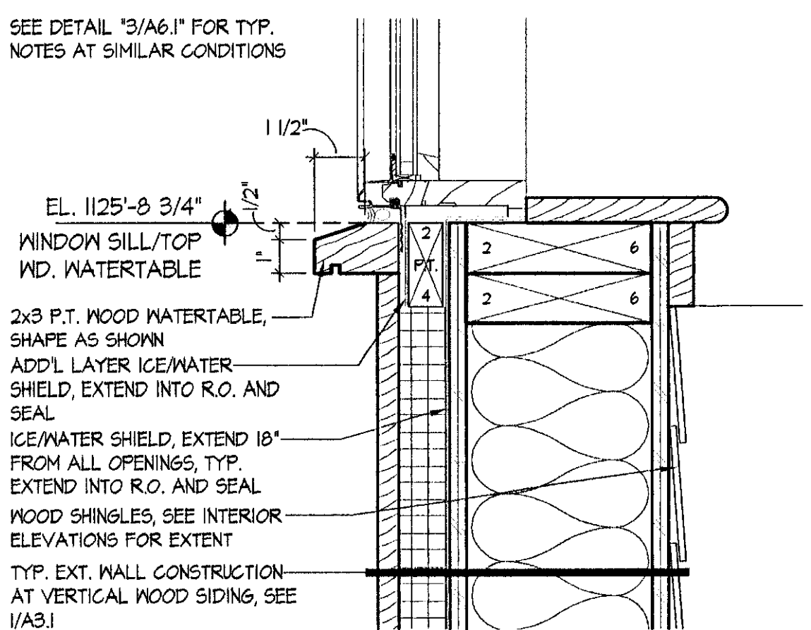
10 FIXED WINDOW SILL @ DORMER SCALE: 3" = 1'-0"
