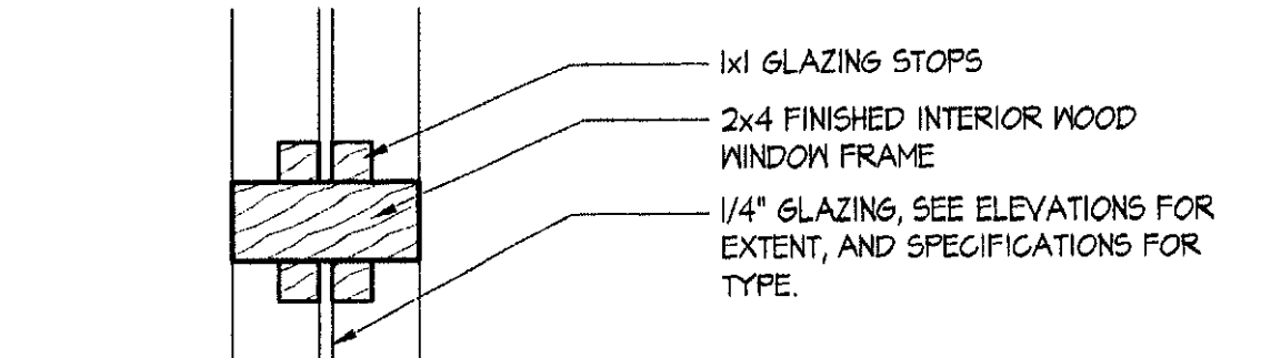
8 INTERIOR WINDOW MULLION SCALE: 3" = 1'-0"
