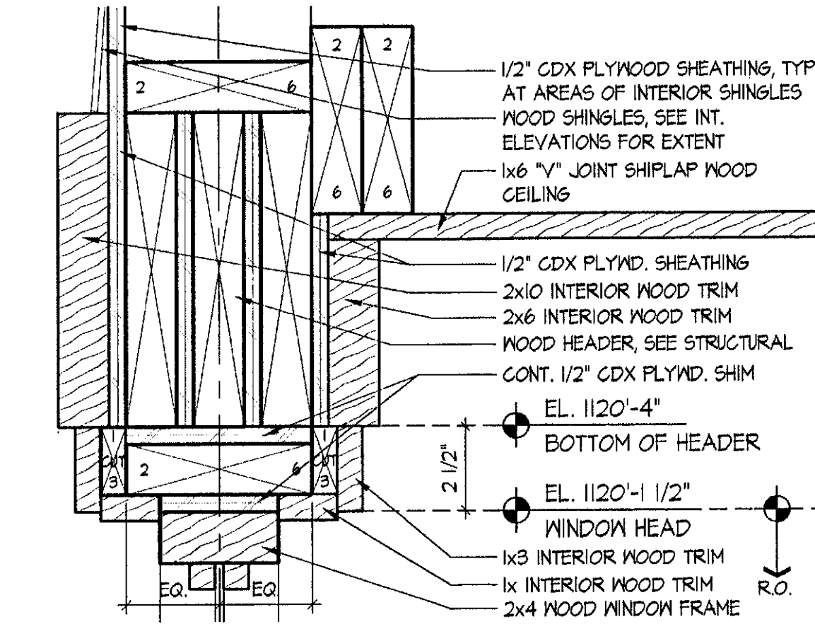
5 INTERIOR WINDOW HEAD SCALE: 3" = 1'-0"
