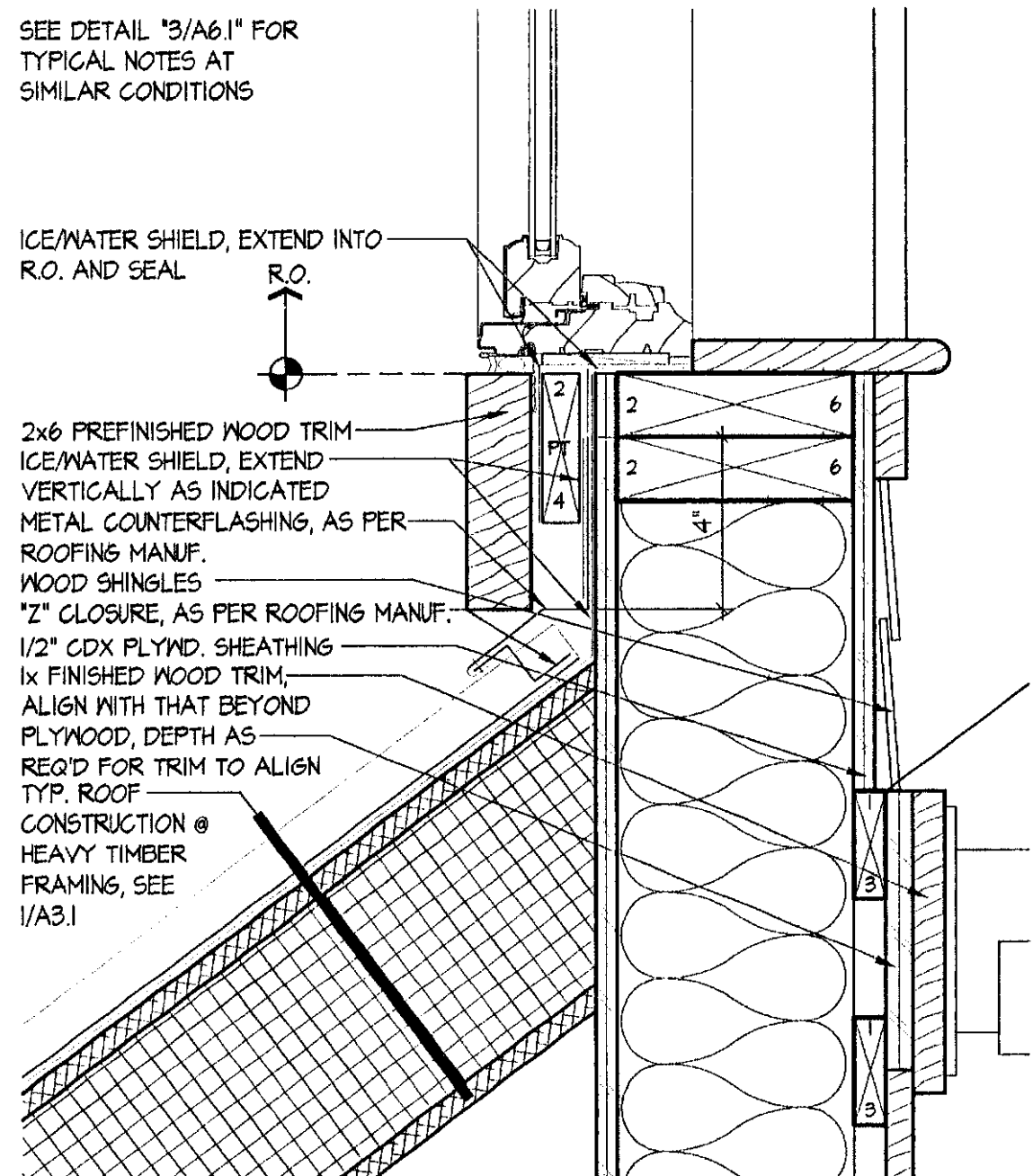
9 FIXED WINDOW SILL @ DORMER SCALE: 3" = 1'-0"
