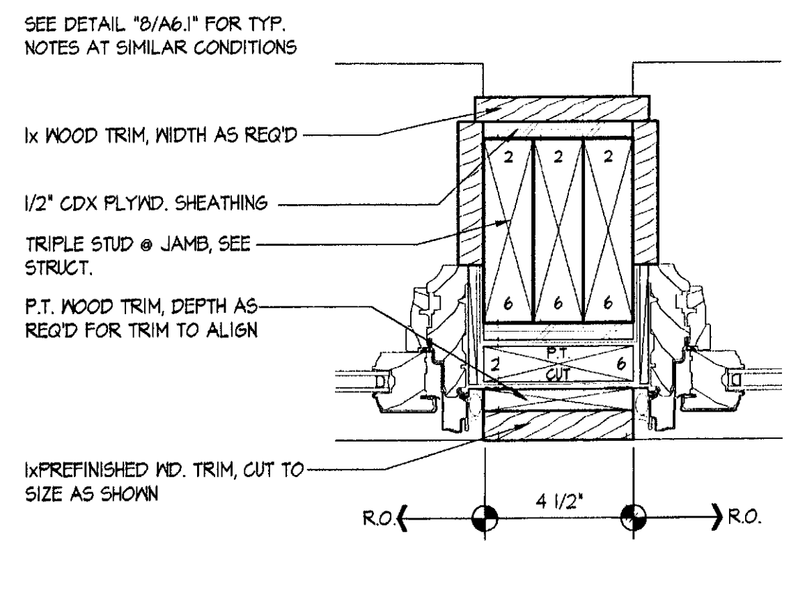
7 FIXED WINDOW JAMB @ DORMER SCALE: 3" = 1'-0"
