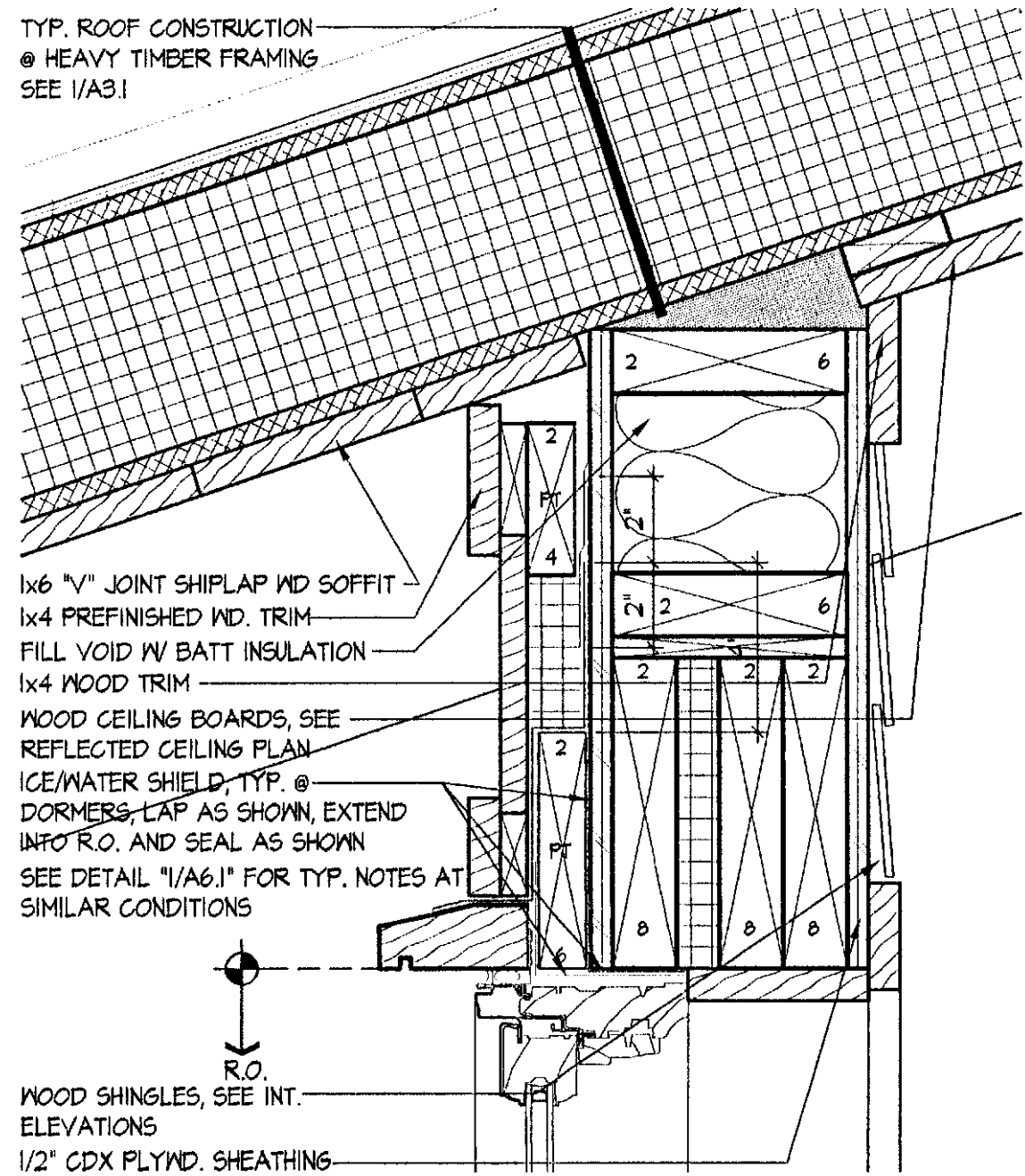
1 FIXED WINDOW HEAD @ DORMER SCALE: 3" = 1'-0"
