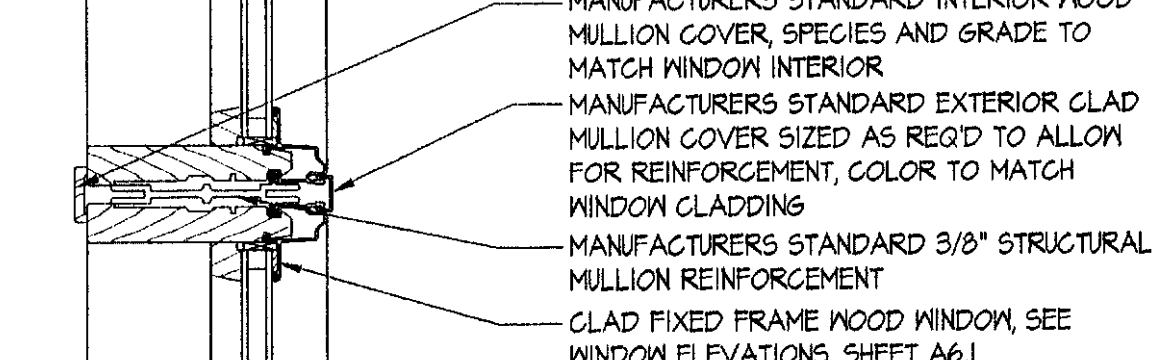
19 TYP. VERTICAL MULLION SCALE: 3" = 1'-0"
